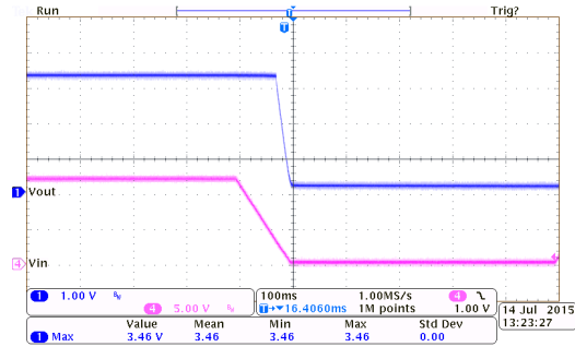
Power Off Response: HT7333-2 ( I_{OUT}=0mA , T_{FALL}=100ms )
