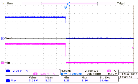
Power Off Response: HT7350-7 ( I_{OUT}=250mA , T_{FALL}=0.1ms )
