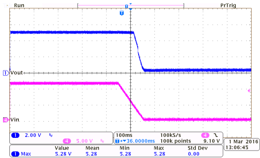
Power Off Response: HT7350-7 ( I_{OUT}=0mA , T_{FALL}=100ms )
