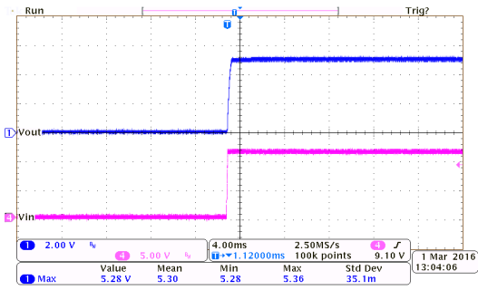
Power On Response: HT7350-7 ( I_{OUT}=250mA , T_{RISE}=0.1ms )
