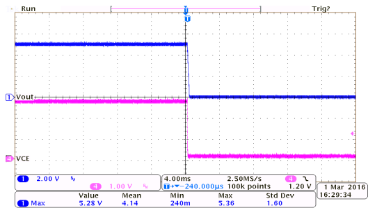
Power Off Response: HT7350-7 ( I_{OUT}=250mA, V_{CE}=2.7V to 0V)
