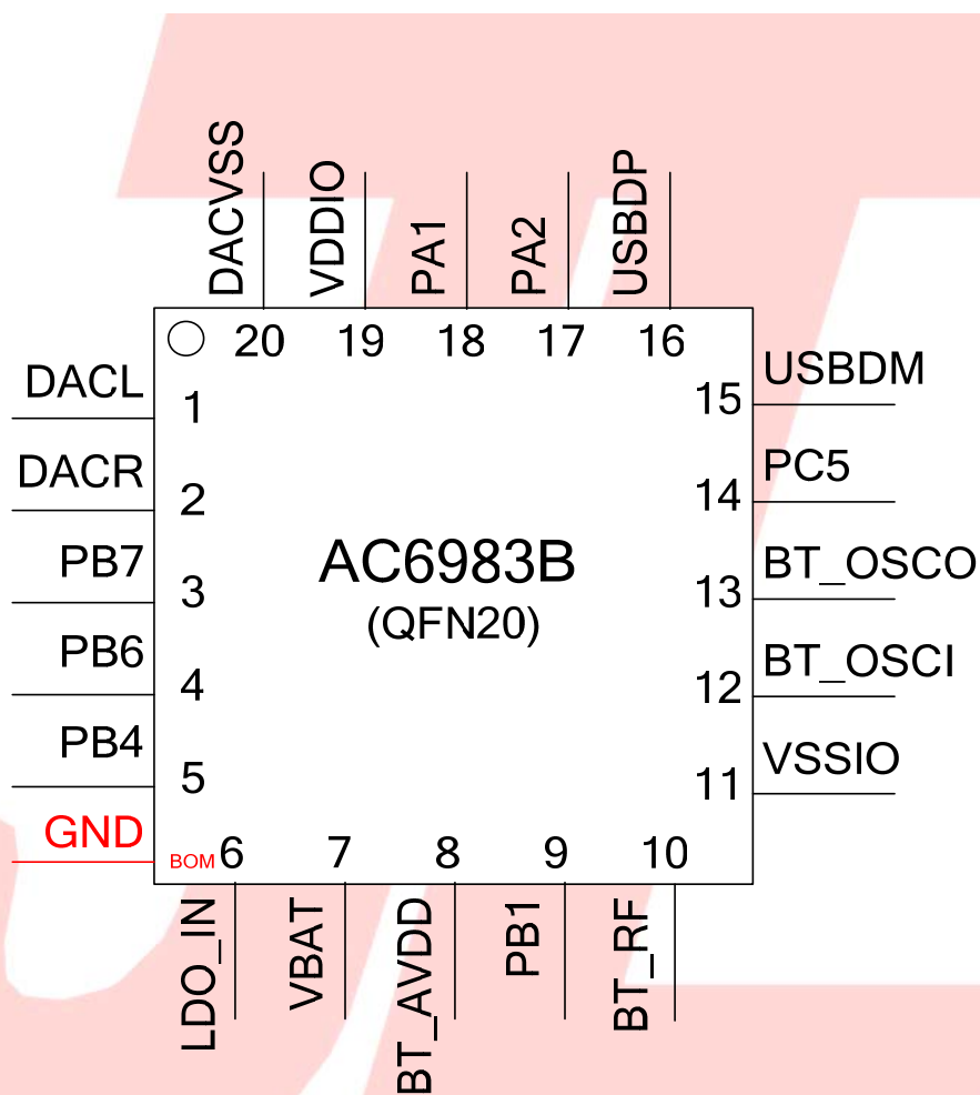
Figure 1-1 AD6983B Package Diagram
