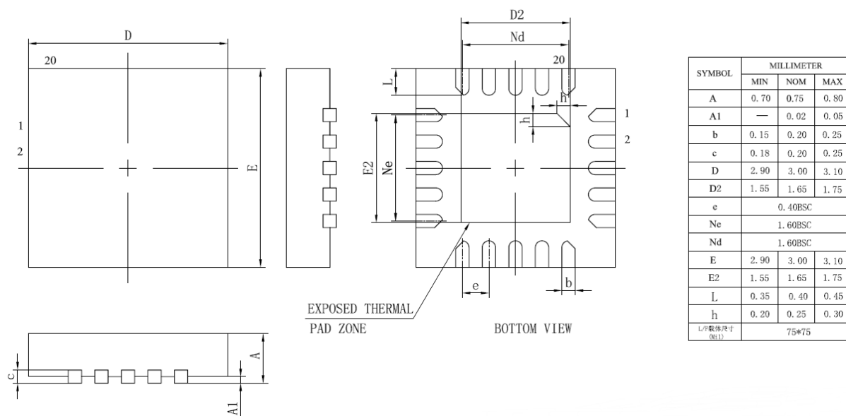
Figure 3-1 AD6983B Package
