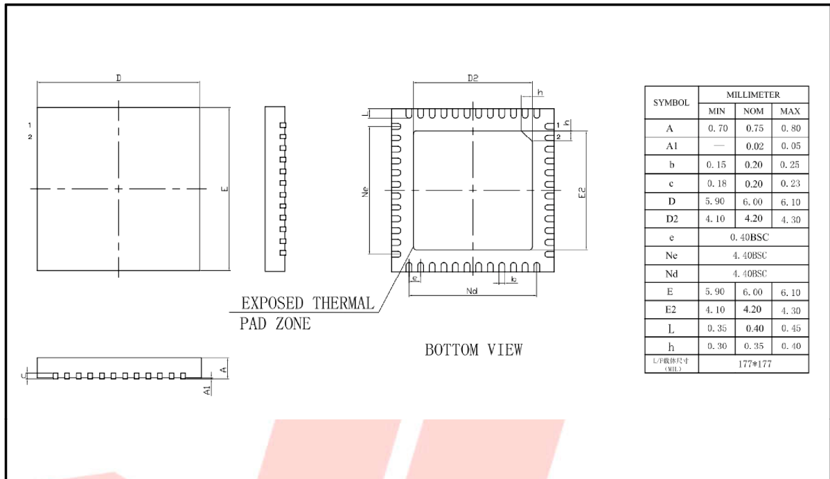
Figure 3-1 AC7911B8_QFN48 Package
