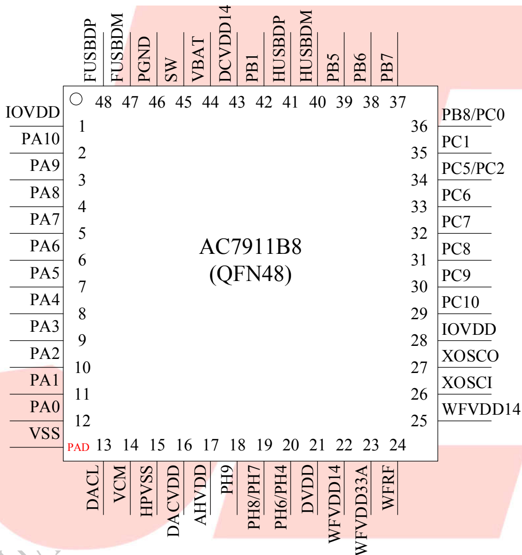
Figure 1-1 AC7911B8_QFN48 Package Diagram
