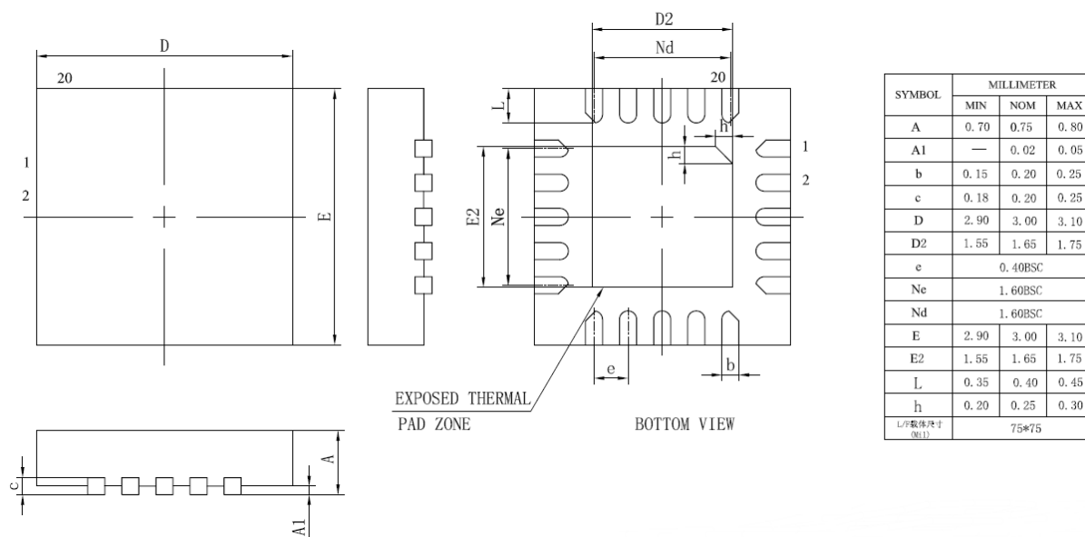
Figure 3-1 AC7003A Package
