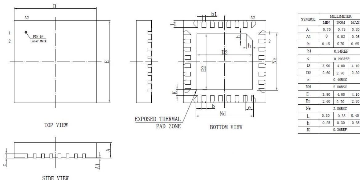
Figure 3-1 JL7006D Package
