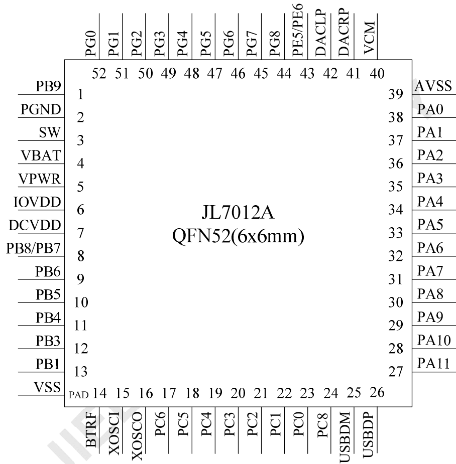
Figure 2-1 JL7012A Package Diagram
