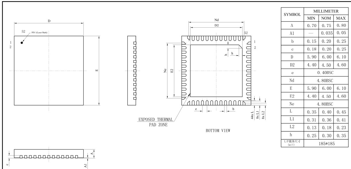
Figure 4-1 JL7012A Package
