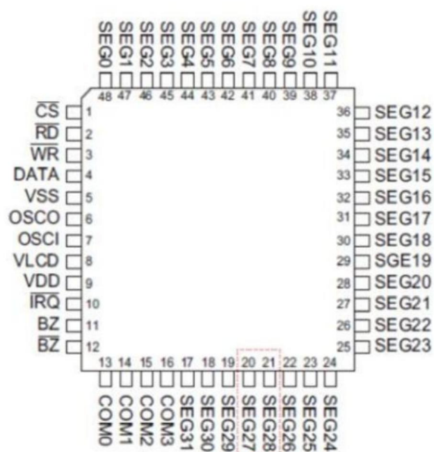
LQFP-48
