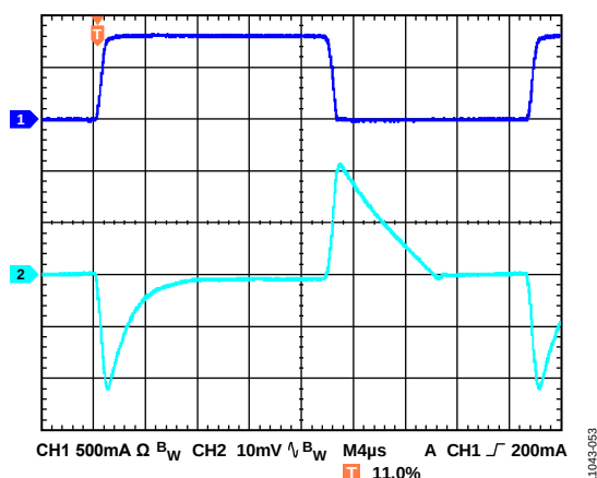
Figure 53. Output Transient Response, V_{\text{OUT}} = 5\text{ V} , C_{\text{OUT}} = 10\ \mu\text{F} , CH1 = Load Current, CH2 = V_{\text{OUT}}
