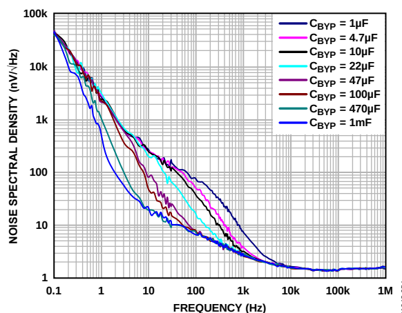
Figure 54. Noise Spectral Density vs. Frequency, C_{\text{BYP}} = 1\ \mu\text{F} to 1 mF
