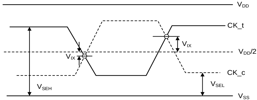
Figure 7-9. V_{IX} Definition (CK)
