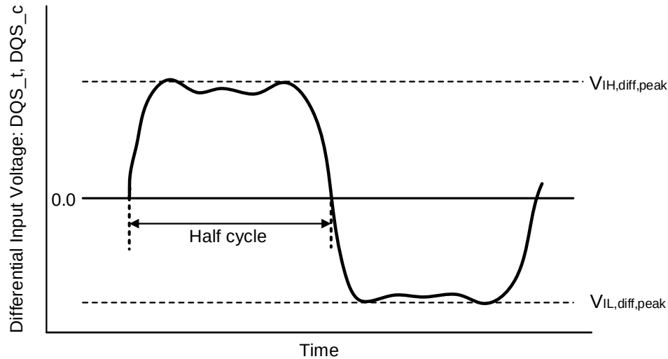
Figure 7-11 Definition of differential DQS Signal AC-swing Level
