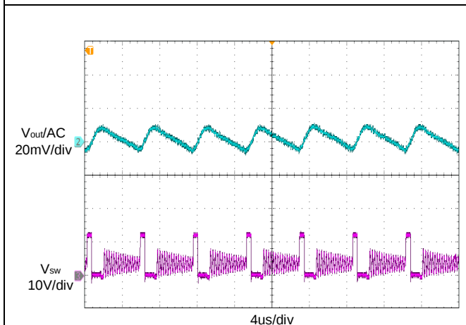
Figure 12. Output Voltage Ripple ( I_{OUT}=100mA )
