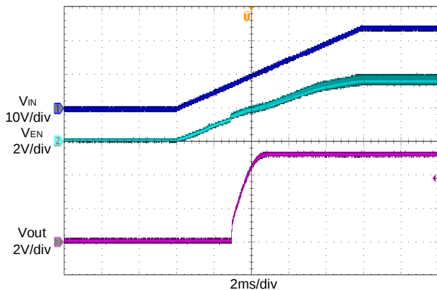
Figure 16. VIN Start-Up without Load
