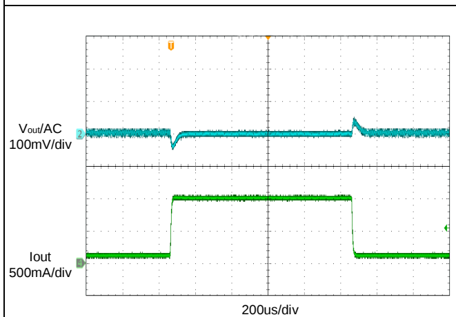
Figure 14. Transient Response (0.1 to 1A)
