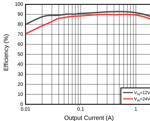
Figure 7. 3.3V Output Efficiency
