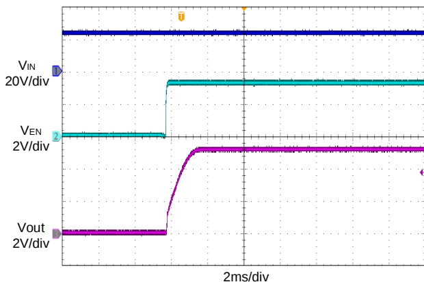
Figure 18. EN Start-Up with Load
