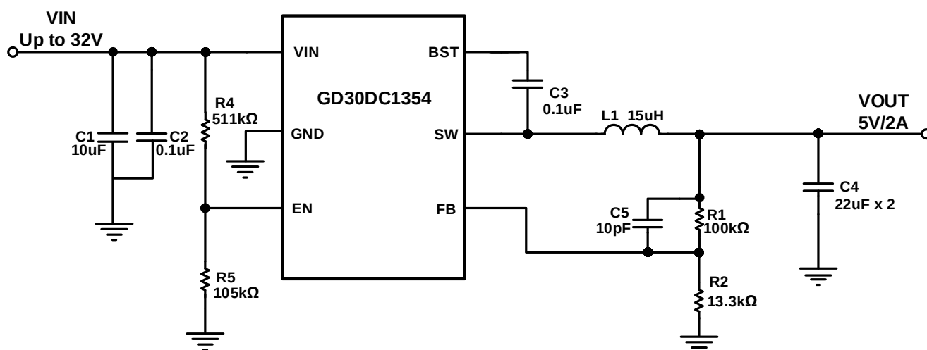
Figure 4. 5V, 2A Reference Design
