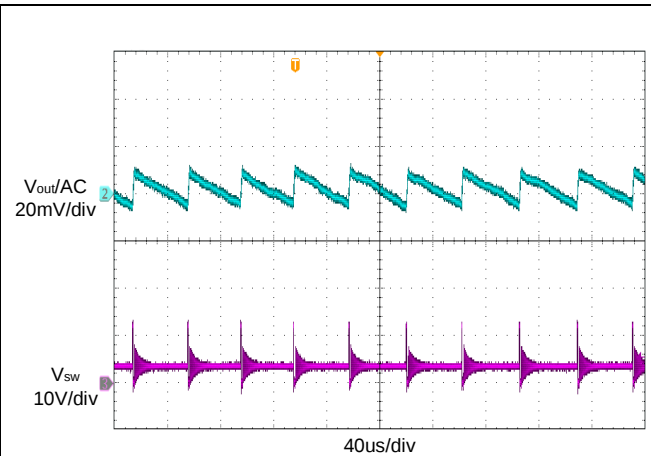
Figure 11. Output Voltage Ripple ( I_{OUT}=10mA )
