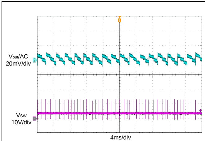
Figure 10. Output Voltage Ripple ( I_{OUT}=0A )
