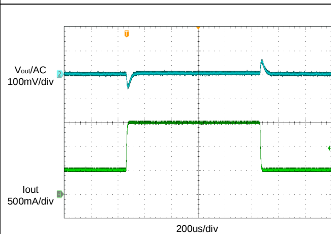
Figure 15. Transient Response (0.5 to 1.5A)
