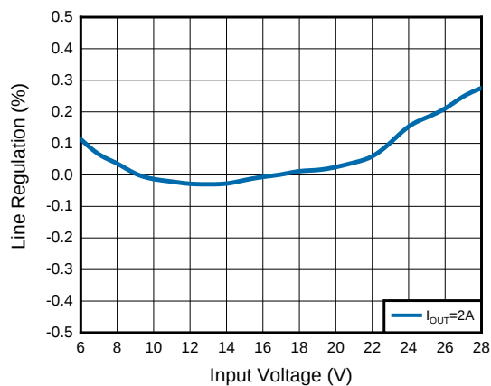
Figure 9. Line Regulation
