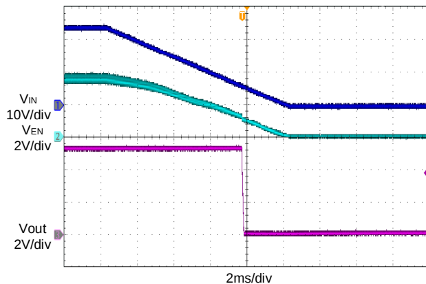
Figure 17. VIN Shut-Down without Load
