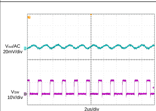
Figure 13. Output Voltage Ripple ( I_{OUT}=2A )
