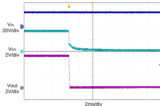
Figure 19. EN Shut-Down with Load
