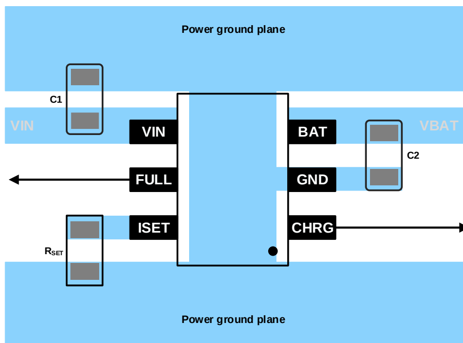
Figure 4. Typical GD30DC1500 Example Layout
