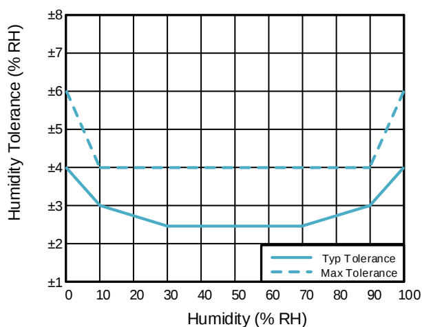
Figure 1. Tolerance of RH @25°C for GD30TSHTV4
