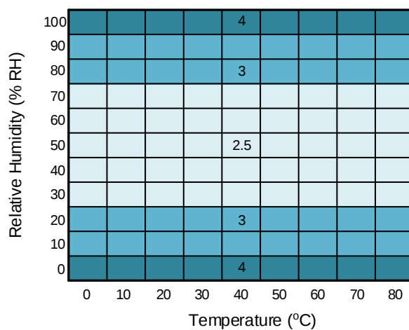
Figure 2. Typical RH Accuracy Tolerance Over Humidity and Temperature for GD30TSHTV4
