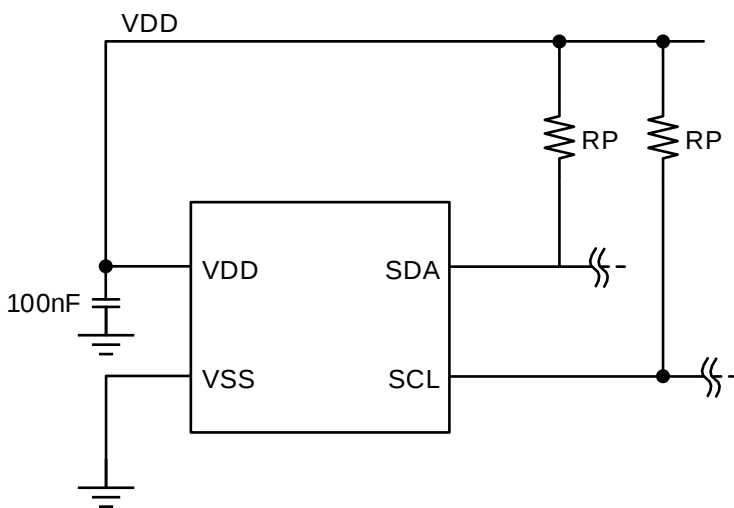
Figure 6. GD30TSHTV4 Reference Circuit
