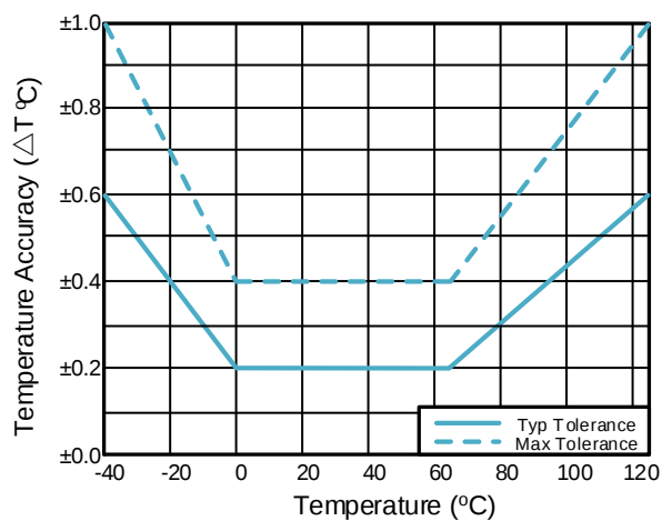
Figure 3. Temperature accuracy of GD30TSHTV4
