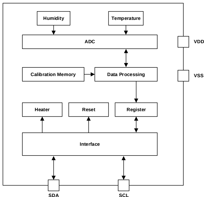
Figure 4. GD30TSHTV4 Block Diagram
