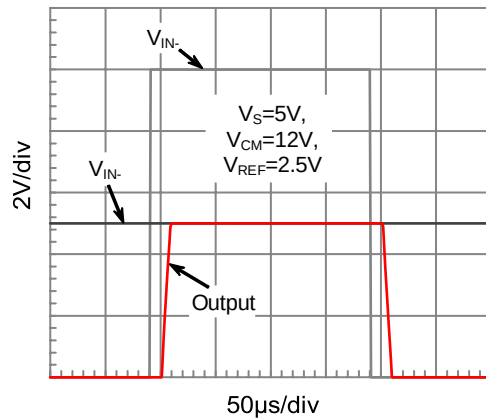
Figure 8. Noninverting Differential Input Overload
