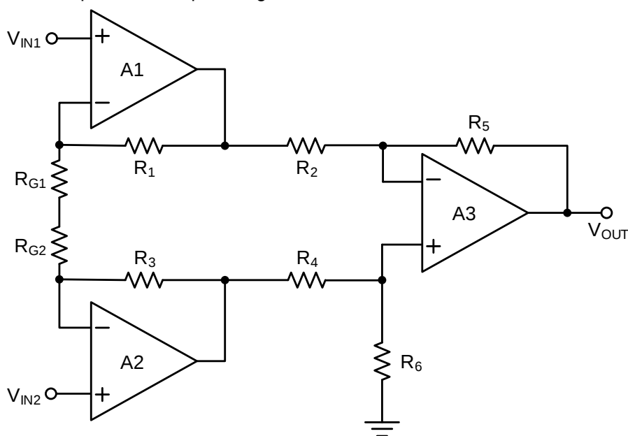
Figure 20. Discrete 3-Op-amp Instrumentation Amplifier
