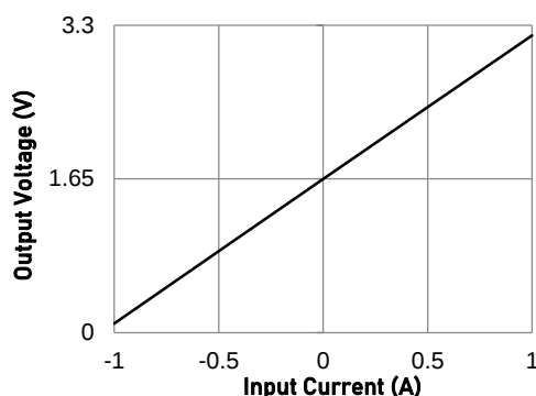
Figure 17. Bidirectional Current-Sensing Circuit Performance: Output Voltage vs. Input Current
