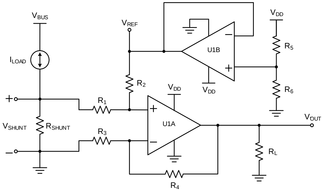
Figure 16. Bidirectional Current-Sensing Schematic
