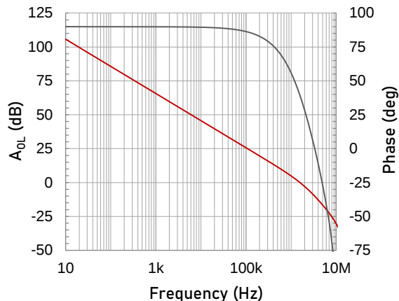
Figure 2. Open Loop Gain and Phase vs. Frequency
