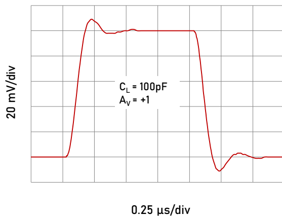
Figure 10. Small Signal Step Response(0.1 step)
