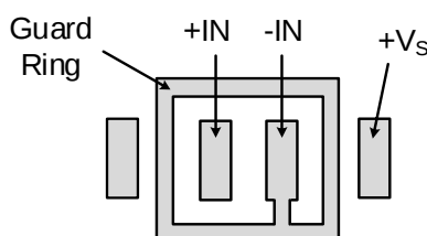
Figure 14. Use a Guard Ring around Sensitive Pins
