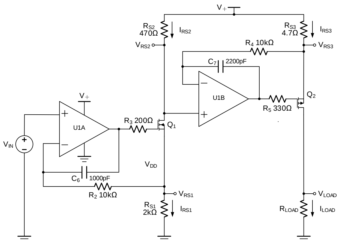
Figure 18. Bidirectional Current-Sensing Schematic
