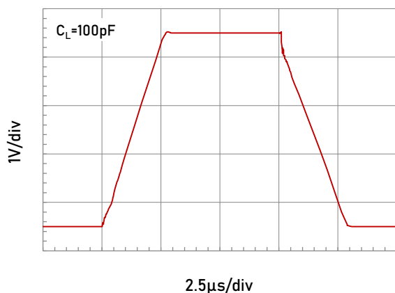
Figure 9. Large Signal Step Response(4V step)
