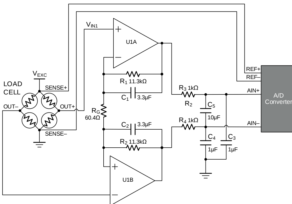
Figure 21. Precision Weigh Scale Measurement System
