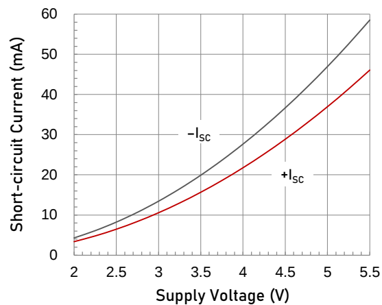
Figure 8. Short-circuit Current vs. Supply Voltage
