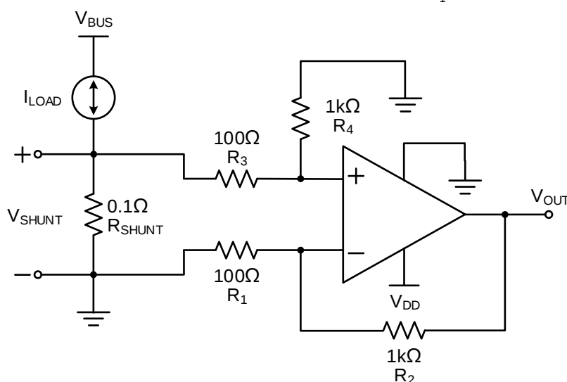
Figure 15. Low Side Current Sensing Circuit
