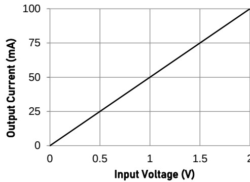
Figure 19. Measured Transfer Function for High-Side V-I Converter
