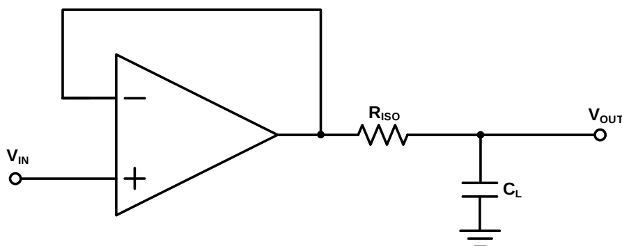
Figure 12. Indirectly Driving Heavy Capacitive Load
