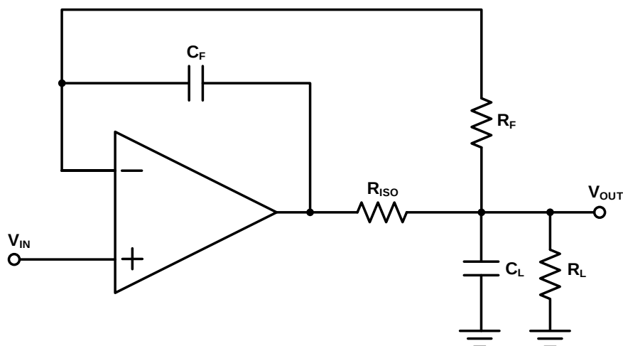
Figure 13. Indirectly Driving Heavy Capacitive Load with DC Accuracy
