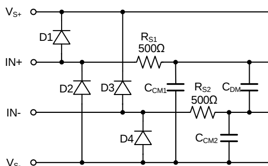
Figure 11. Input EMI Filter and Clamp Circuit
