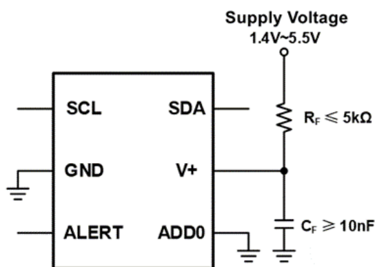
Figure 10. Noise Reduction Techniques
