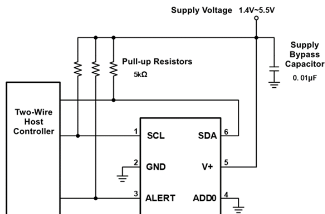
Figure 9. Typical Connections of the GD30TS112N
