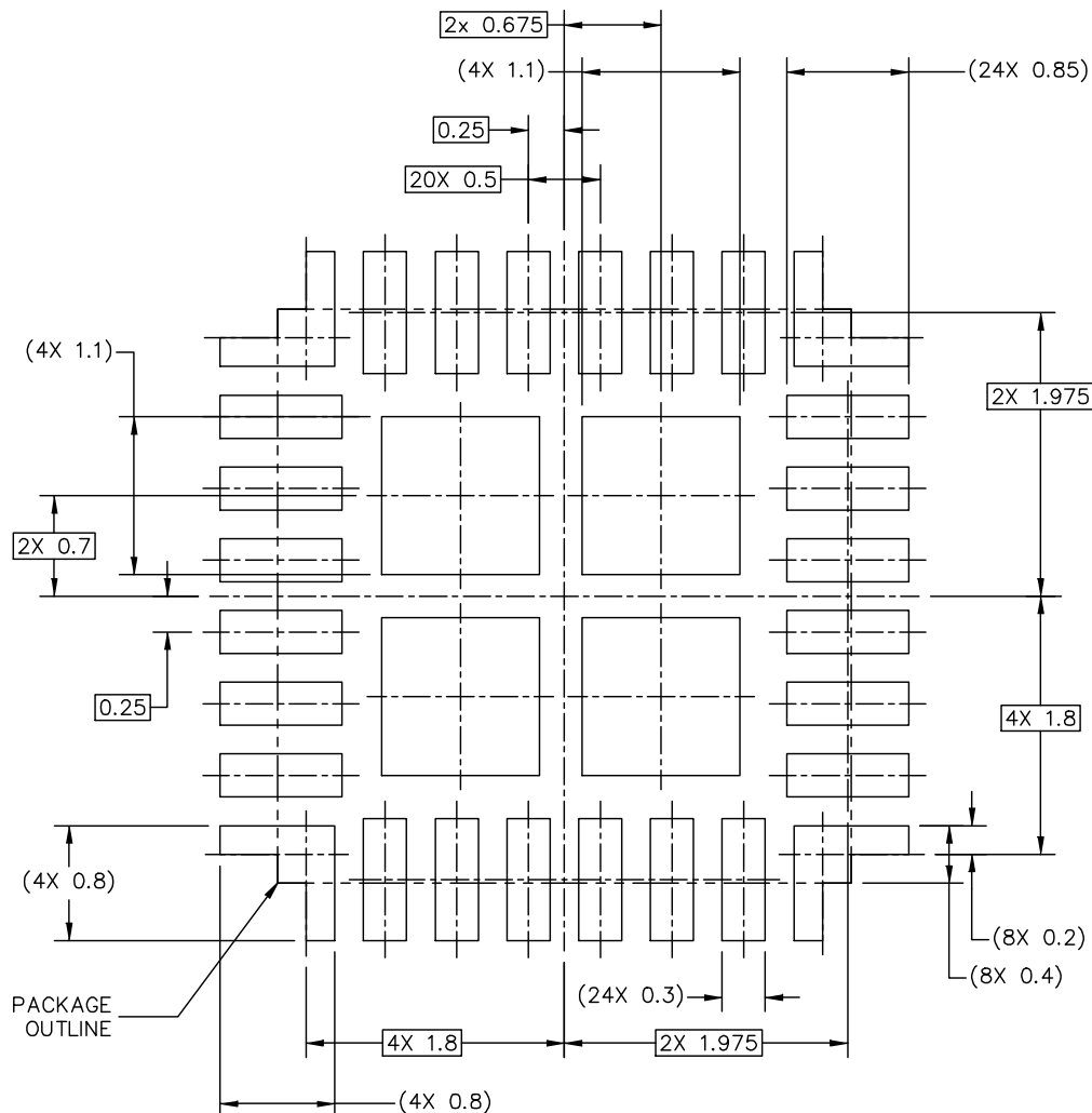
Figure 12. Reflow soldering footprint part3 for HQFN24 (SOT1931-1(D))
