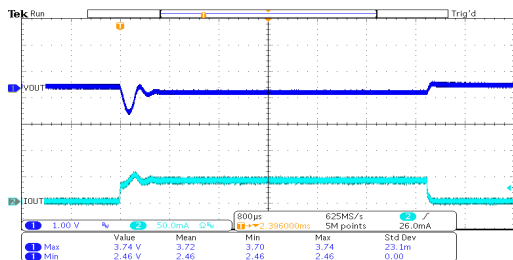
负载瞬态响应: HT7533-1 (V IN =5.3V, I OUT =0mA~40mA)
