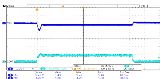
负载瞬态响应: HT7550-1 (V IN =7V, I OUT =0mA~40mA)
