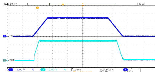
开关响应: HT7550-1 ( V_{IN}=12V , I_{OUT}=0mA , TRISE=TFALL=100ms )
