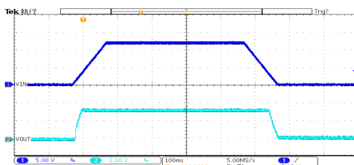
开关响应: HT7533-1 ( V_{IN}=12V , I_{OUT}=0mA , TRISE=TFALL=100ms )
